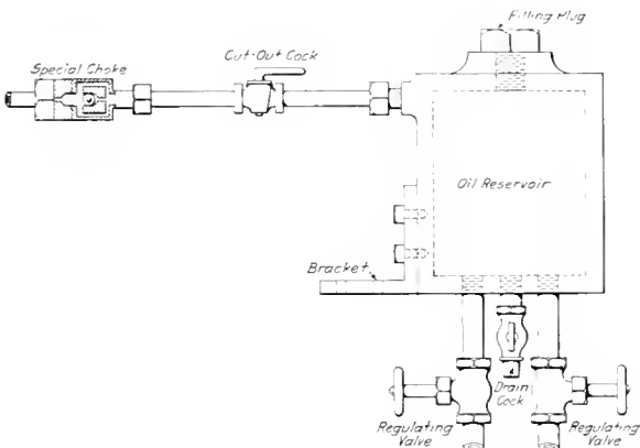
Lubricator for Cross-Compound Air Compressors
